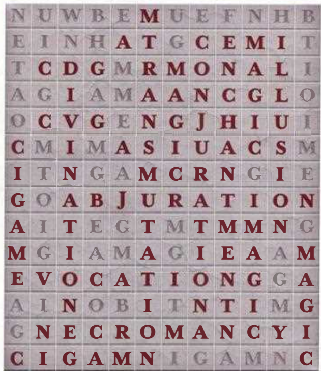
DIAGRAM 4.1: RECKLESS STEPS PUZZLE SOLUTION
